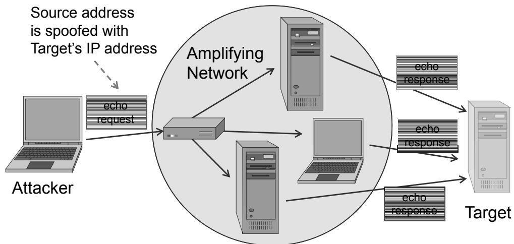
Figure 19: A smurf attack uses a misconfigured network to amplify traffic intended to overwhelm the bandwidth of a target.
