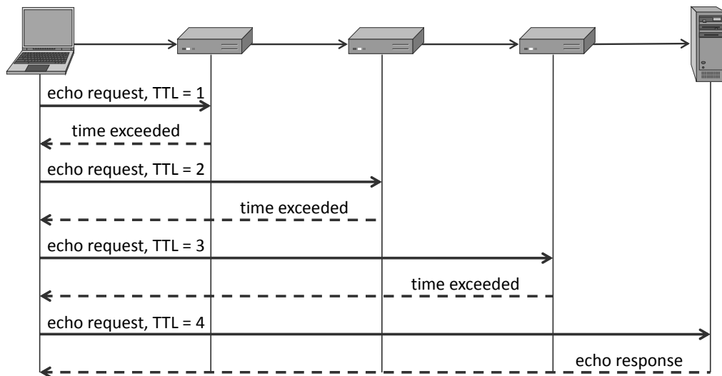
Figure 11: The traceroute utility.
