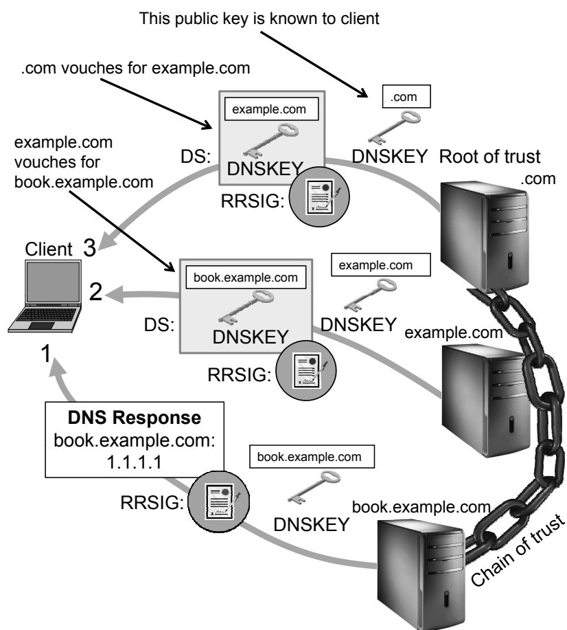
Figure 9: A DNSSEC response and the chain of trust that validates it. In this case, book.example.com returns a signed DNS response along with its public key, example.com sends its public key and a signed DS record validating the public key of book.example.com , and .com sends its public key and a signed DS record validating the public key of example.com . The client can trust this chain, since it knows the public key of .com . (computer tower) © tatniz/Shutterstock; (key) © Igor Nazarenko/Shutterstock
