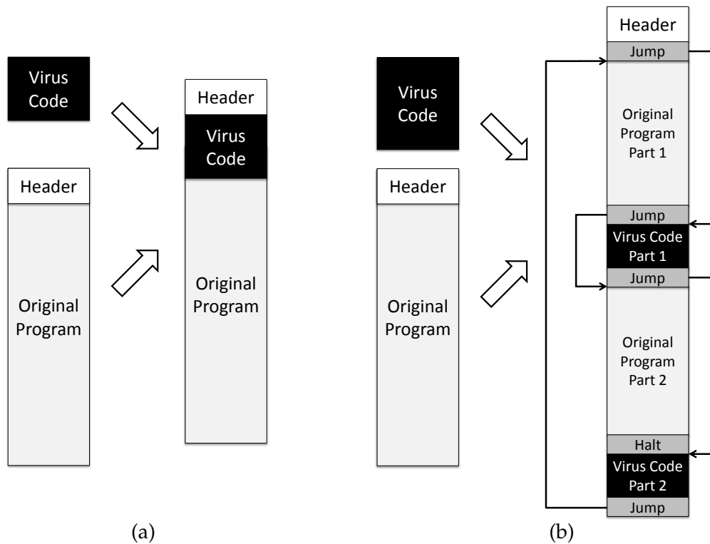
Figure 4: How a virus injects itself into a program file: (a) A simple injection at the beginning of a program. (b) A more complex injection that splits the virus code into two parts and injects them at different points in the program. Jump instructions are used to begin execution with the virus code and then pass control to the original program code.
