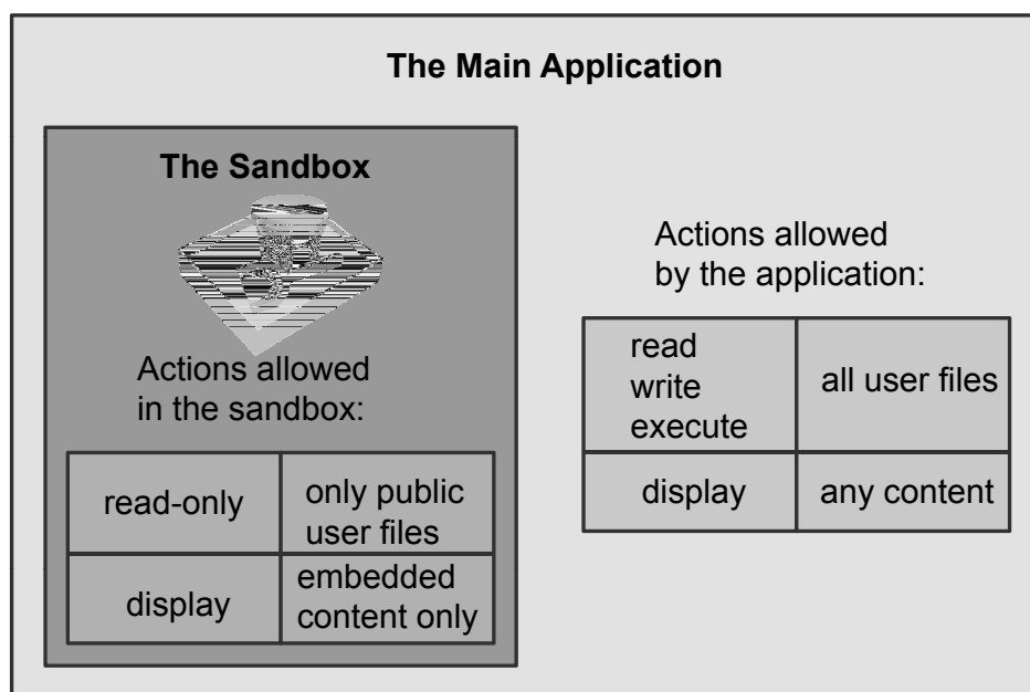
Figure 15: Actions restricted to a sandbox.
