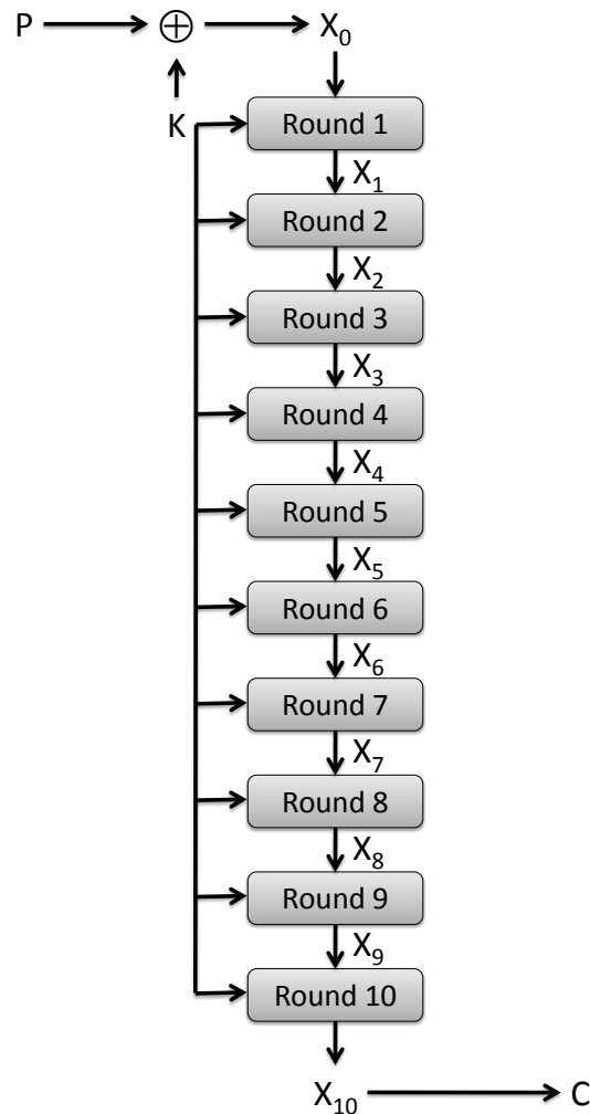
Figure 5: The AES rounds.
