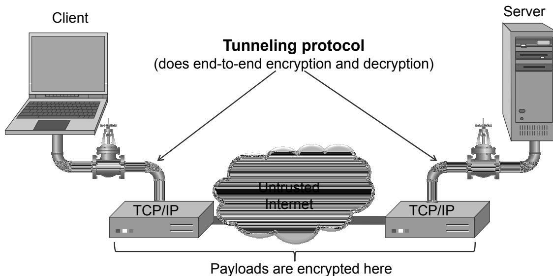
Figure 14: Tunneling protocols provide end-to-end encryption of TCP/IP communication between a client and a server. © Plart/Shutterstock
