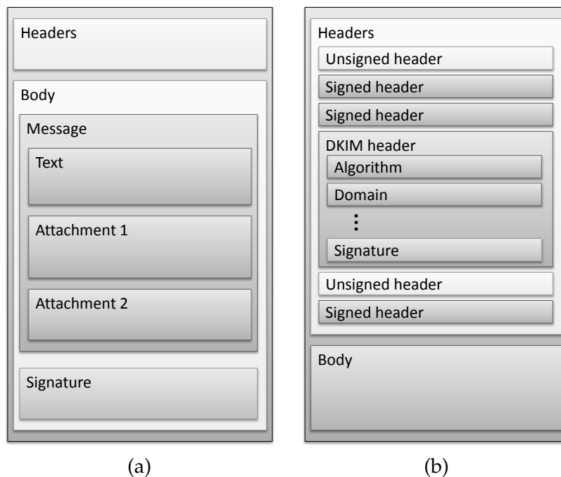
Figure 6: Digitally signed email messages: (a) Structure of an S/MIME message, where the signature part refers to the rest of the message body, but not to the headers. (b) Structure of a DKIM message, where the signature in the DKIM header field refers to the message body and selected headers.
