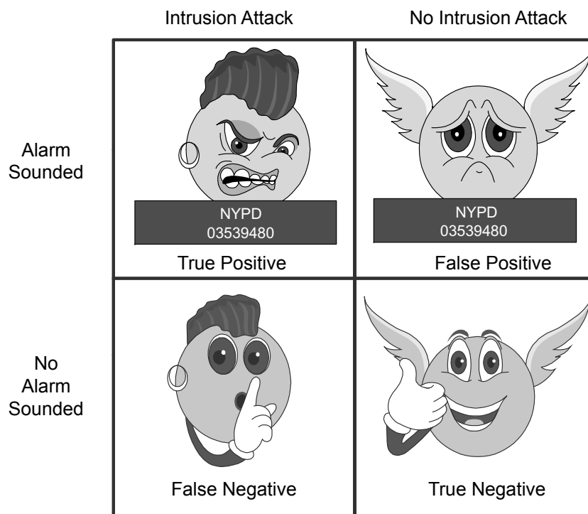
Figure 18: The four conditions for alarm sounding by an intrusion detection system.
