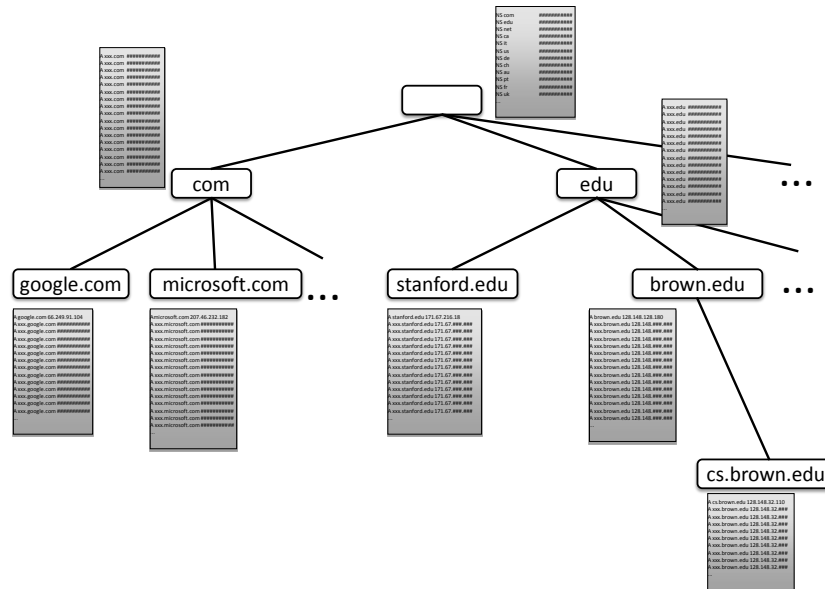
Figure 2: The hierarchical organization of authoritative name servers. Each name server stores a collection of records, each providing the address of a domain or a reference to an authoritative name server for that domain.
