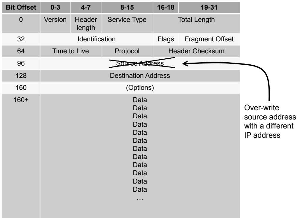
Figure 12: How IP spoofing works. The source address in the header of an IP packet is simply overwritten with a different IP address from the actual source. Note the header checksum field also needs to be updated.
