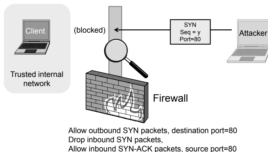
Figure 12: A stateless firewall dropping TCP sessions initiating an HTTP connection with a request from outside the trusted internal network.
