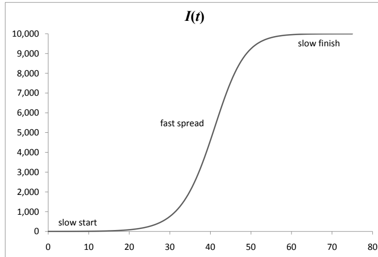
Figure 8: The epidemic model of the spread of a worm. The chart shows the number of infected hosts I(t) as a function of time for a total population of N = 10,000 hosts and infection rate \beta = 0.000025 , starting from a single host.
