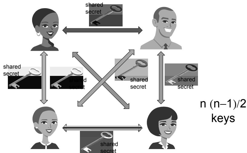
Figure 9: Pairwise confidential communication among n users with a symmetric cryptosystem requires n(n - 1)/2 distinct keys, each shared by two users and kept secret from the other users. (key) © Igor Nazarenko/Shutterstock; (avatars) © Moneca/Shutterstock
