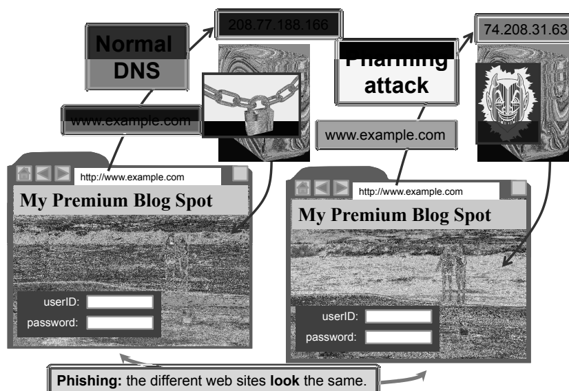
Figure 5: A pharming attack that maps a domain name to a malicious server, which then performs a phishing attack by delivering a web page that looks the same as the real one, to trick people into entering their userIDs and passwords. (Image by Karen Goodrich; used with permission.) With permission of Brown University, Providence, RI; (devil) © SFerdon/Shutterstock; (padlock with chains) © 3dpixs.com/Fotolia, LLC–Royalty Free; (computer tower) © tatniz/Shutterstock
