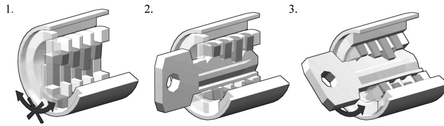
Figure 3: Opening a wafer tumbler lock: (1) Closed lock. Image included with permission [71]. (2) After inserting the key. Image included with permission [72]. (3) Open lock. Image included with permission [73].
