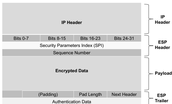
Figure 16: The ESP header.
