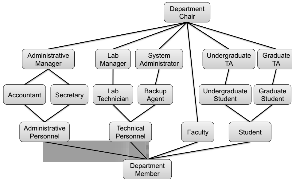
Figure 7: Example of hierarchy of roles for a computer science department.
