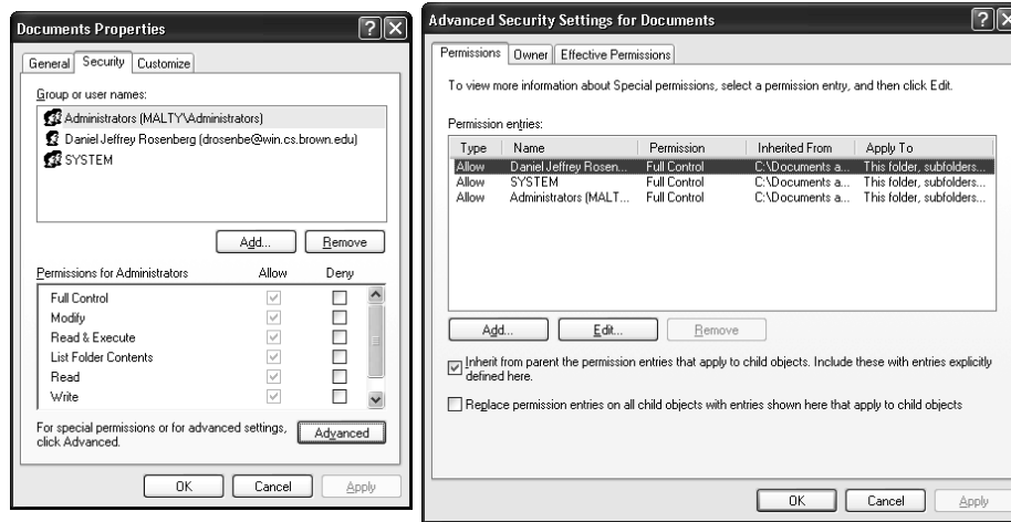
Figure 13: Customizing file permissions in Windows XP. Microsoft® and Windows® are registered trademarks of the Microsoft Corporation in the U.S.A. and other countries. Screen shots and icons reprinted with permission from the Microsoft Corporation. This book is not sponsored or endorsed by or affiliated with the Microsoft Corporation.
