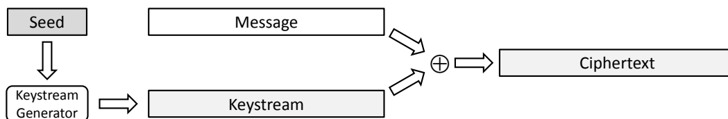
Figure 24: Encryption with a stream cipher.
