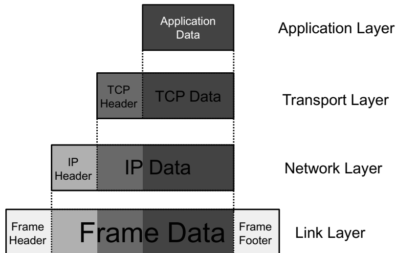
Figure 2: Packet encapsulation in the link, network, transport, and application layers of the Internet protocol stack. Each packet from a higher layer becomes the data for the next lower-layer packet, with headers added to the beginning, and, for frames, a footer added at the end.
