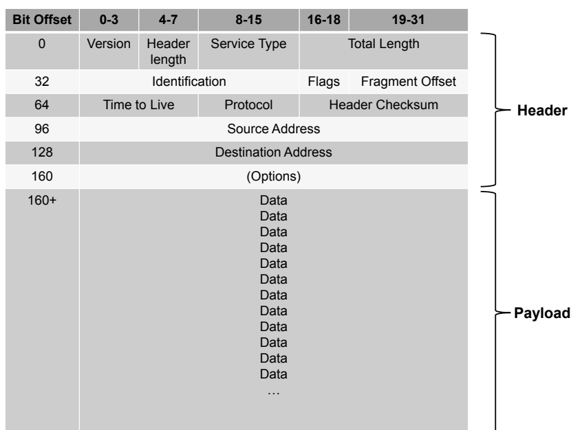
Figure 10: Format of an IPv4 packet.
