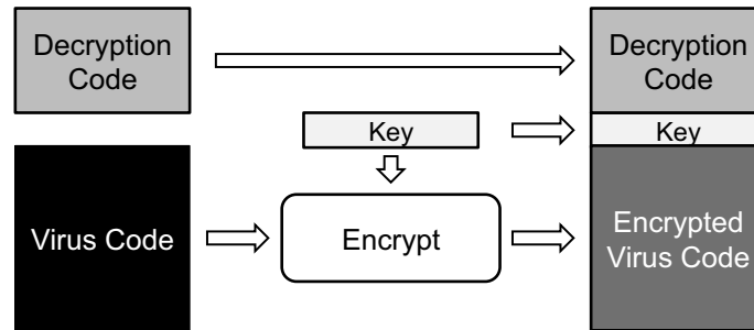
Figure 5: How an encrypted virus is structured.
