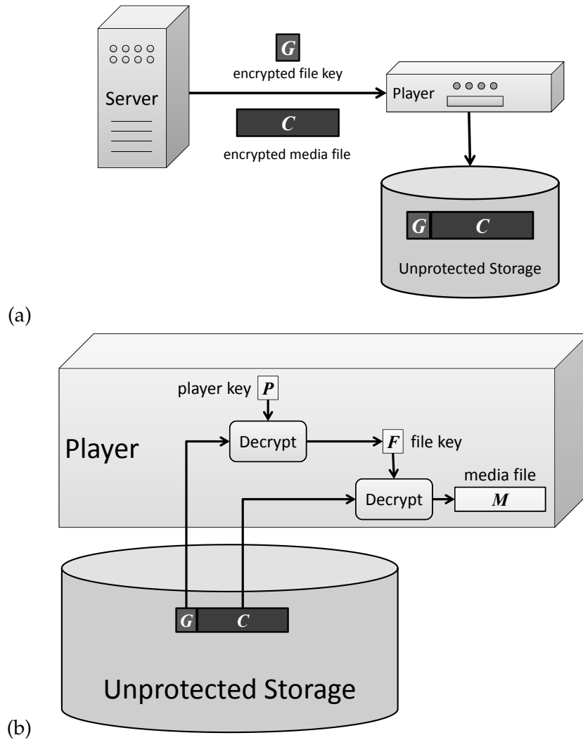
Figure 12: A simple DRM scheme for media files: (a) the media server sends to the player the media file encrypted with the file key and the file key encrypted with the player key; (b) the player first decrypts the file key using the player key and then decrypts the media file with the file key.
