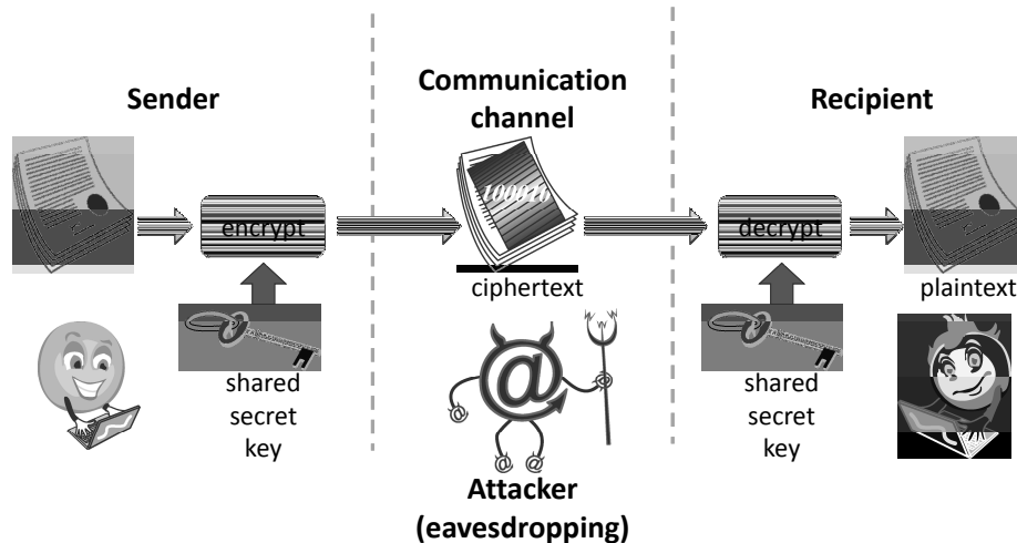
Figure 8: A symmetric cryptosystem, where the same secret key, shared by the sender and recipient, is used to encrypt and decrypt. An attacker who eavesdrops the communication channel cannot decrypt the ciphertext (encrypted message) without knowing the key.
