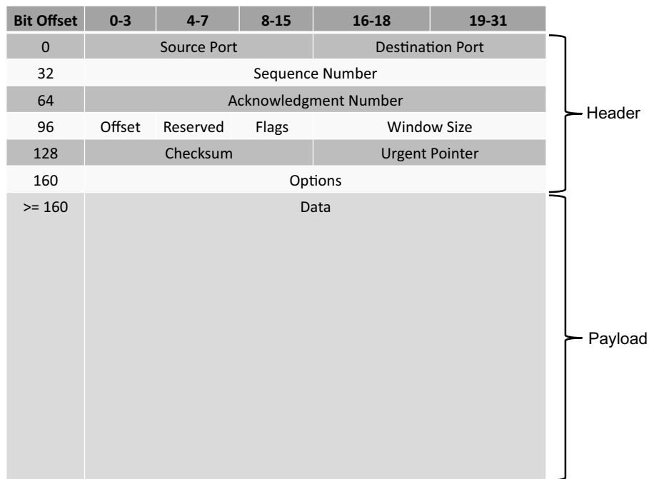
Figure 14: Format of a TCP packet.
