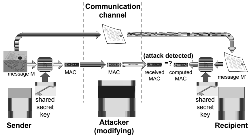
Figure 15: Using a message authentication code to verify the integrity of a message. © Igor Nazarenko/Shutterstock
