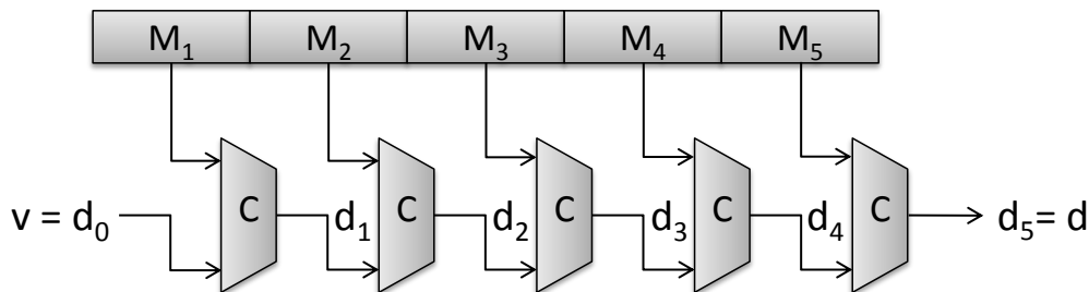
Figure 12: The Merkle-Damgård construction.
