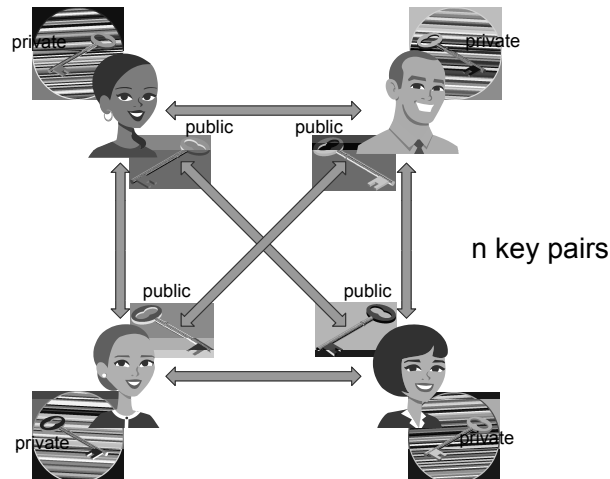
Figure 11: Pairwise confidential communication among n users with a public-key cryptosystem requires n key pairs, one per user. (key) © Igor Nazarenko/Shutterstock; (avatars) © Moneca/Shutterstock
