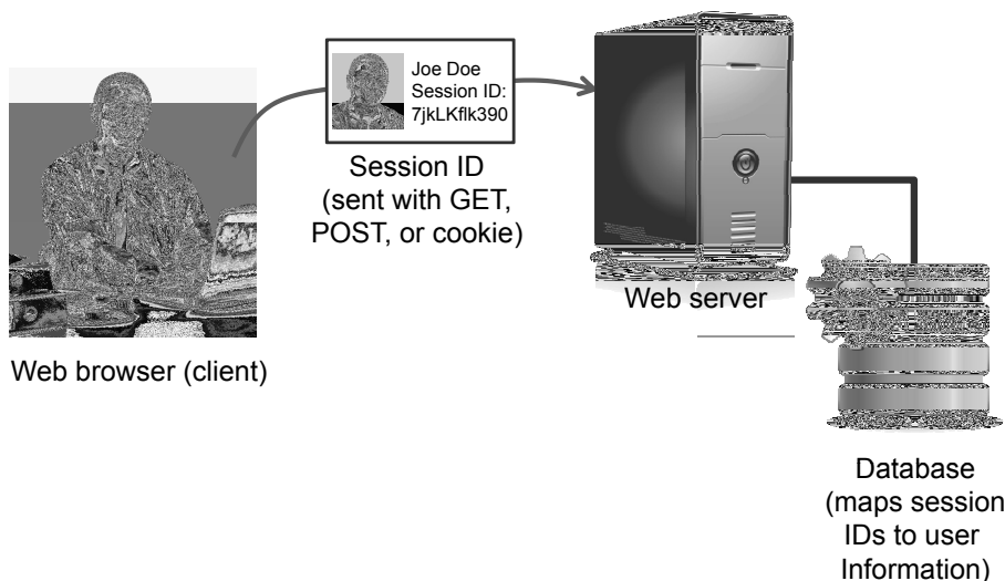
Figure 12: Creating a web session using a session ID. ("Joe Doe") © EDHAR/Shutterstock; ("Web server") © Viktor Gmyria/Shutterstock; ("Database") © frbird/Shutterstock
