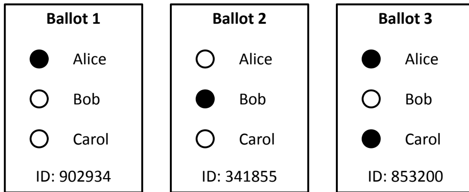
Figure 15: In this ThreeBallot election, the voter votes for Alice by marking two of the three ballots at random for Alice, and votes against Bob and Carol by marking only one ballot at random for each of these candidates.
