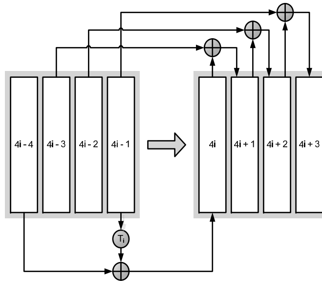
Figure 15: The key schedule for AES encryption.
