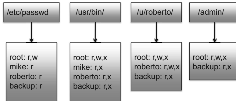
Figure 5: The access control lists (ACLs) corresponding to the access control matrix of Table 1. We use the shorthand notation of r=read, w=write, and x=execute.
