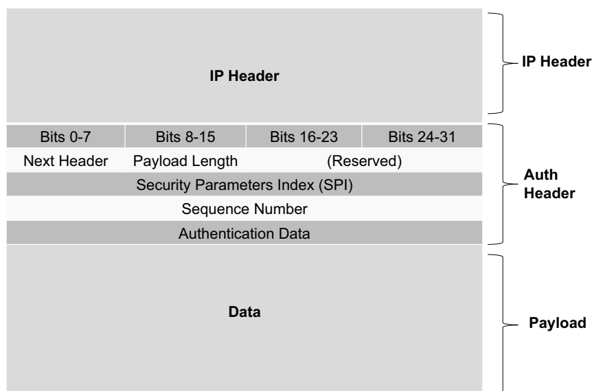
Figure 15: The authentication header.
