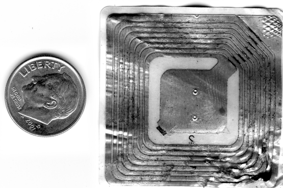
Figure 11: An RFID tag, taken from a DVD package, together with a dime to show size. Photo by Dan Rosenberg included with permission.
