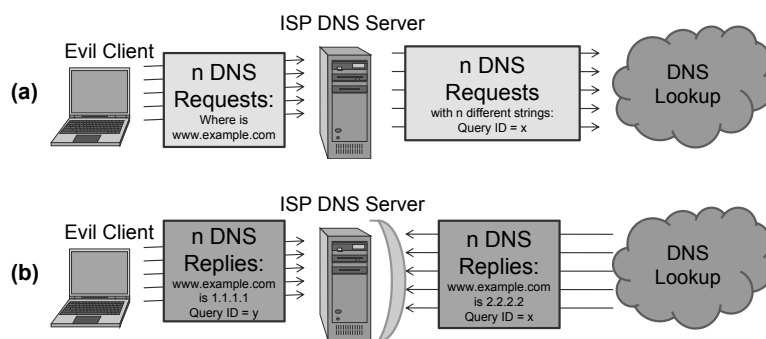
Figure 7: A DNS cache poisoning attack based on the birthday paradox: (a) First, an attacker sends n DNS requests for the domain she wishes to poison. (b) The attacker sends n corresponding replies for her own request. If she successfully guesses one of the random query IDs chosen by the ISP DNS server, the response will be cached.
