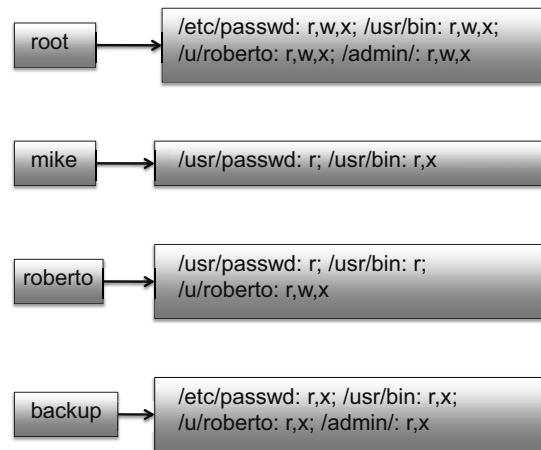
Figure 6: The capabilities corresponding to the access control matrix of Table 1. We use the shorthand notation of r =read, w =write, and x =execute.
