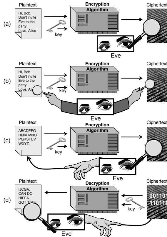
Figure 2: Types of attacks: (a) Ciphertext-only attack. (b) Known-plaintext attack. (c) Chosen-plaintext attack. (d) Chosen-ciphertext attack. (“Eve”) © Zara’s Gallery/Shutterstock; (“Ciphertext”) © Lukiyanova Natilia/Shutterstock; (key) © Igor Nazarenko/Shutterstock
