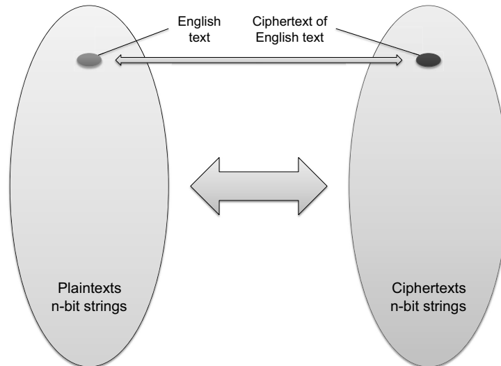
Figure 14: Natural-language plaintexts are a very small fraction of the set of possible plaintexts. This fraction tends to zero as the plaintext length grows. Thus, for a given key, it is hard for an adversary to guess a ciphertext that corresponds to a valid message.
