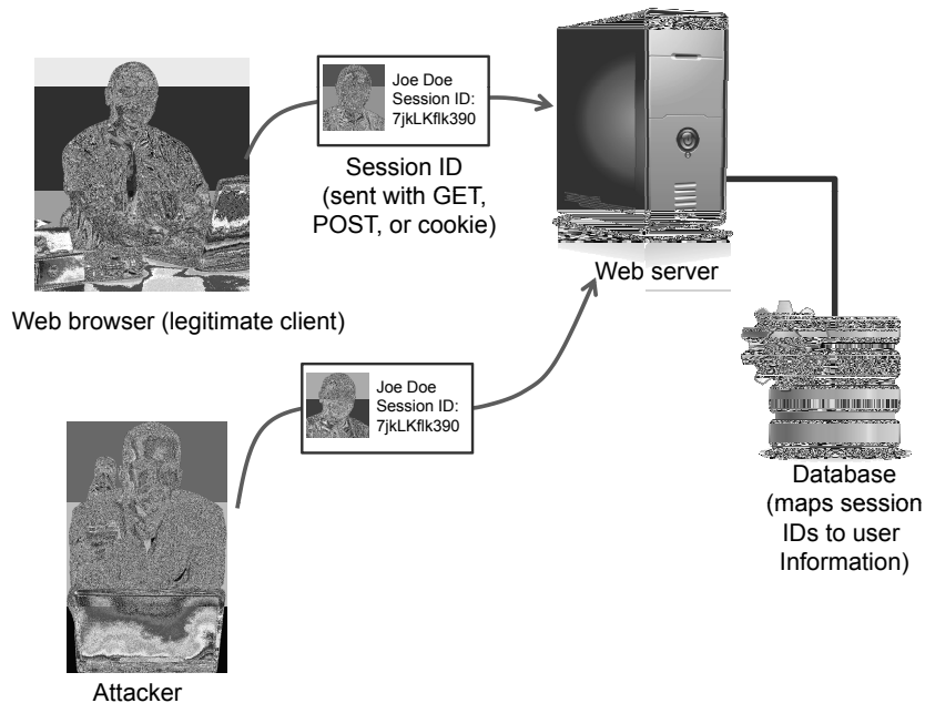
Figure 13: A session hijack attack based on a stolen session ID. (“Joe Doe”) © EDHAR/Shutterstock; (“Web server”) © Viktor Gmyria/Shutterstock; (“Database”) © frbird/Shutterstock; (“Attacker”) © dragon_fang/Shutterstock
