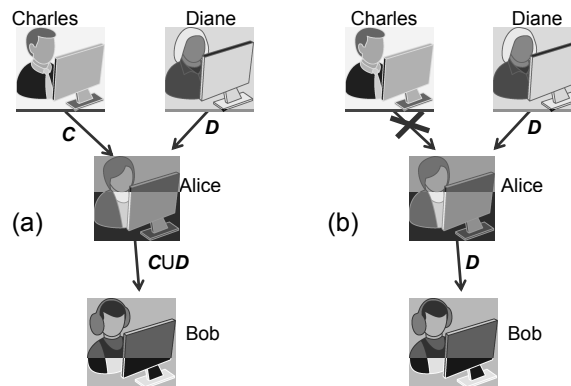
Figure 3: How database privileges can be visualized with a directed diagram: (a) First, two administrators, Charles and Diane, each grant Alice two sets of privileges, C and D , after which Alice grants those privileges to Bob, giving him the set of rights in the union, C \cup D . (b) If Charles subsequently revokes the set of privileges, C , he granted to Alice, then the privileges Bob inherited indirectly from Charles, through Alice, should also be revoked, leaving Bob with just the privileges in D .
