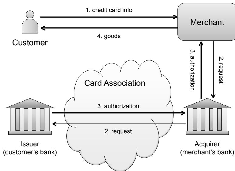
Figure 10: The authorization phase in online credit card processing. (“Card issuing bank,” “Merchant’s bank”/bank) © Zlatko Guzmic/Shutterstock; (“Customer”) © Vallentin Vassileff/Shutterstock; (“Card issuing bank”/credit cards) © Sergil Koroiko/Shutterstock; (“Merchant’s bank”/money bags) © Sferdon/Shutterstock; (“Merchant’s website”) © Lenny712/Shutterstock
