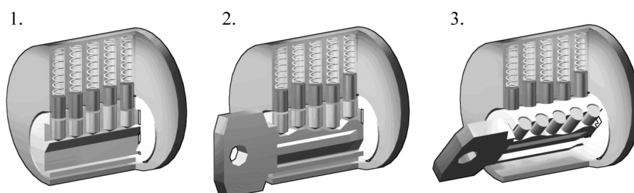
Figure 1: A pin tumbler lock: (1) When a key is not present, the pin stacks are pushed down by the springs so that the driver (top) pins span the plug and the outer casing, preventing the plug from rotating. Image included with permission [108]. (2) When the correct key is inserted, the ridges of the key push up the pin stacks so that the cuts of the pin stacks are aligned with the shear line. Image included with permission [75]. (3) The alignment of the cuts with the shear line allows the plug to be rotated. Image included with permission [76].
