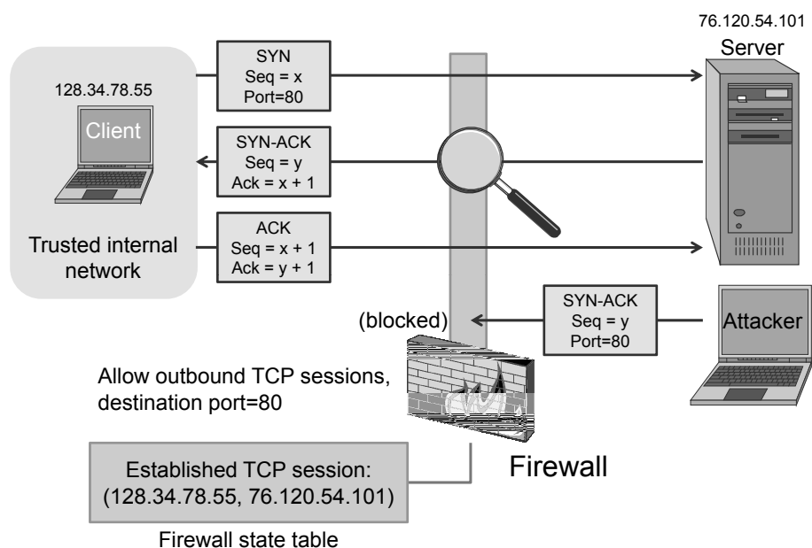
Figure 13: A stateful firewall configured to allow TCP web sessions (port 80) with a request coming from inside the trusted internal network.
