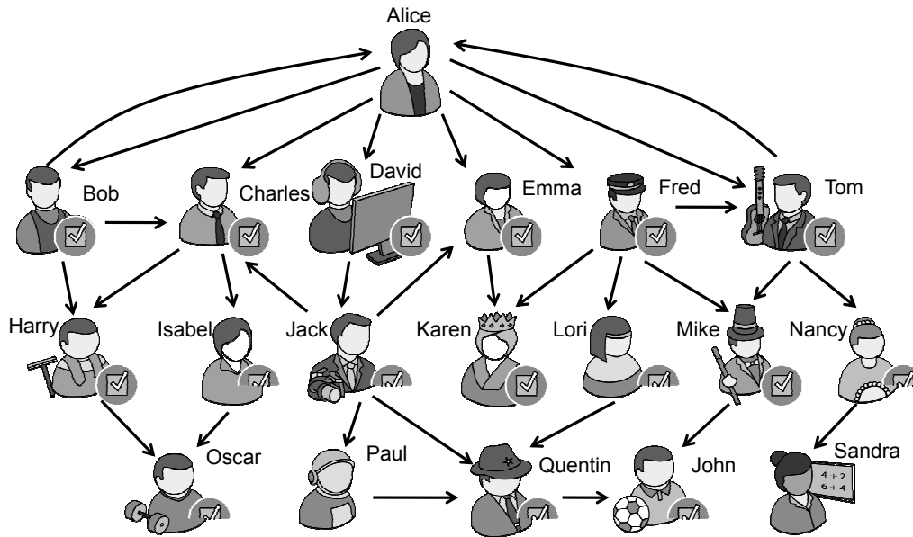
Figure 5: A web of trust in PGP. A directed edge from A to B indicates that A signs B 's key. A full check mark indicates a key Alice fully trusts and a half check mark indicates a key that Alice partially trusts. People without a check mark or with half check mark have no keys that Alice trusts.
