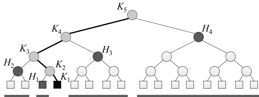
Figure 13: Key tree for player revocation. The black player, which is associated with the solid-filled leaf, stores keys K_1, K_2, K_3, K_4, and K_5 . To revoke the black player, keys H_1, H_2, H_3, and H_4 are used to encrypt replacements for keys K_2, K_3, K_4, and K_5 .
