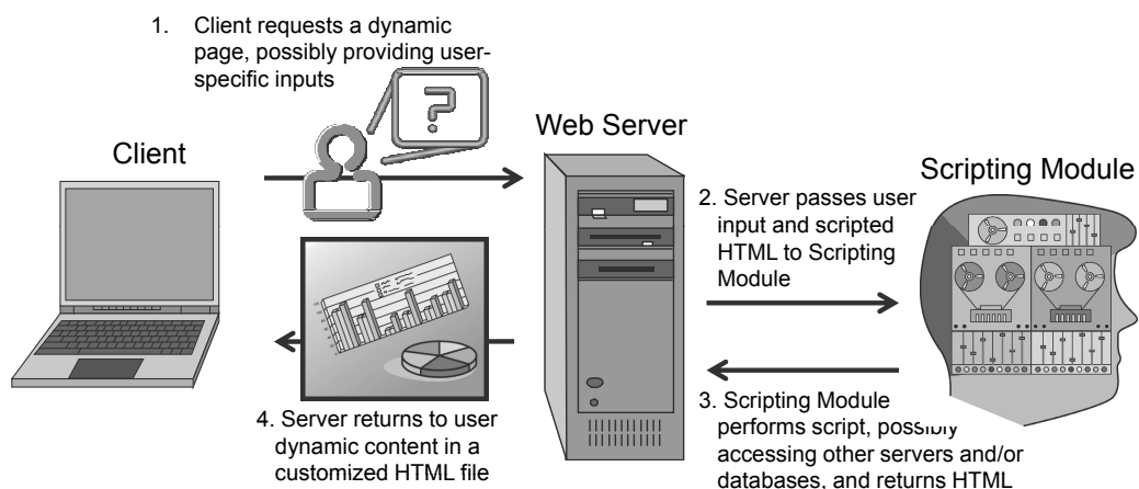
Figure 19: Actions performed by a web server to produce dynamic content for a client user.
