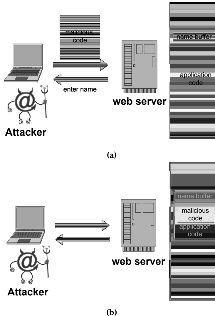
Figure 16: A buffer overflow attack on a web server. (a) A web server accepts user input from a name field on a web page into an unchecked buffer variable. The attacker supplies as input some malicious code. (b) The malicious code read by the server overflows the buffer and part of the application code. The web server now runs the malicious code.
