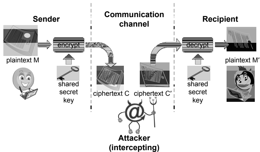
Figure 13: A man-in-the-middle attack where the adversary modifies the ciphertext and the recipient decrypts the altered ciphertext into an incorrect message. © Igor Nazarenko/Shutterstock
