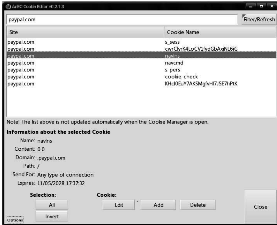
Figure 11: The contents of a cookie viewed using a Firefox cookie editing plugin. The name and content fields correspond to the key-value pair of the cookie. The domain name .paypal.com specifies that this cookie is valid for this top-level domain and all subdomains, and the path / indicates that it applies to the root directory of the site. Finally, the send for value indicates that this is not a secure cookie, and the expiration date specifies when this cookie will be automatically deleted.
