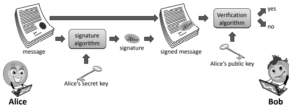
Figure 13: The digital signing process for Alice and the signature verification process for Bob.
