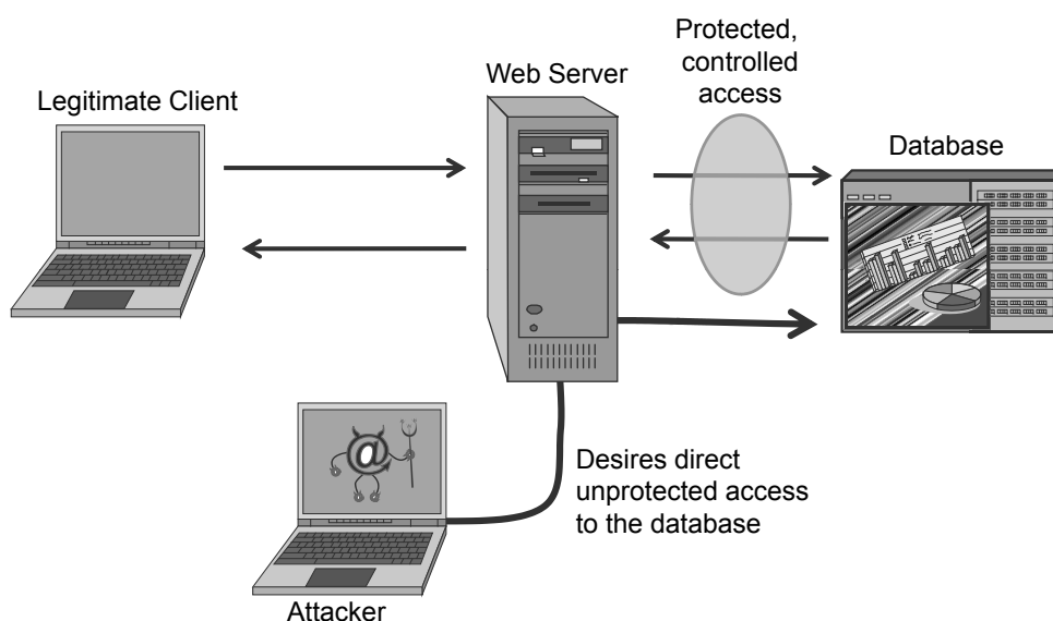
Figure 20: A model for user interactions with a web server that uses a database. All database queries are performed via the web server, and direct access to the database by the user is prohibited. The attacker wants to break through these protections to use the web server to gain direct access to the database.
