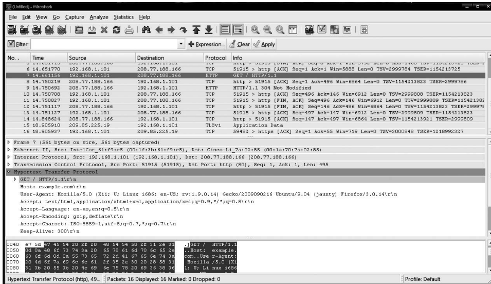
Figure 13: An example use of the Wireshark packet sniffing tool. Here, the packet associated with an HTTP request to www.example.com has been captured and analyzed.
