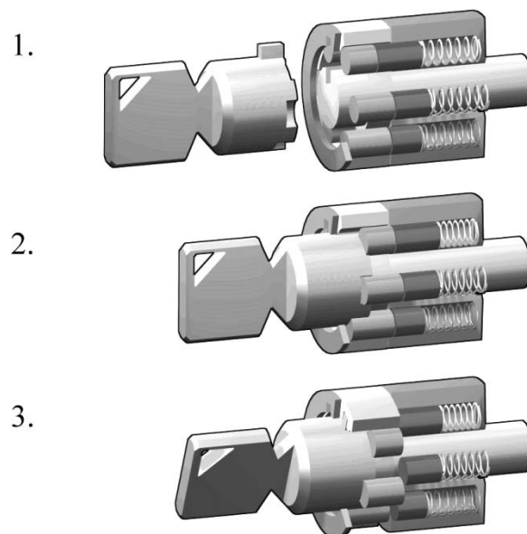
Figure 2: Opening a tubular lock: (1) Closed lock. Image included with permission [68]. (2) After inserting the key. Image included with permission [69]. (3) Open lock. Image included with permission [70].
