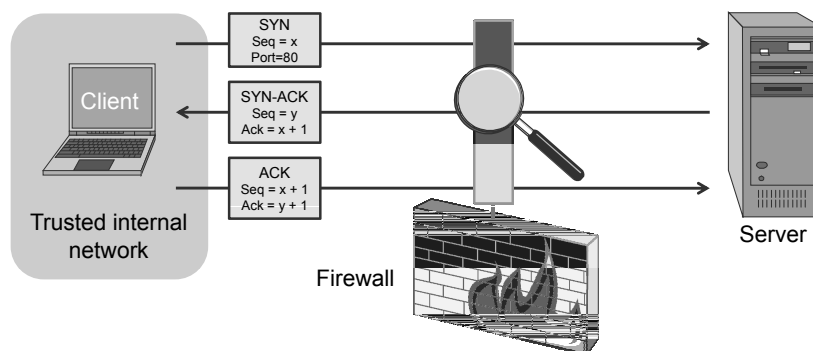
Figure 11: A stateless firewall allowing TCP sessions initiating an HTTP connection (port 80) with a request from the trusted internal network.
