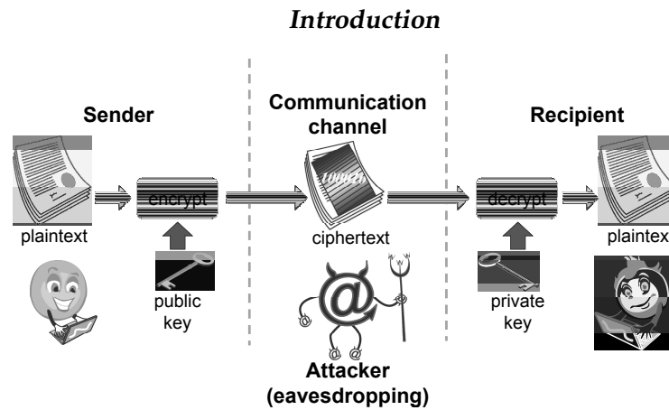
Figure 10: In a public-key cryptosystem, the sender uses the public key of the recipient to encrypt and the recipient uses its private key to decrypt. An attacker who eavesdrops the communication channel cannot decrypt the ciphertext (encrypted message) without knowing the private key. © Igor Nazarenko/Shutterstock
