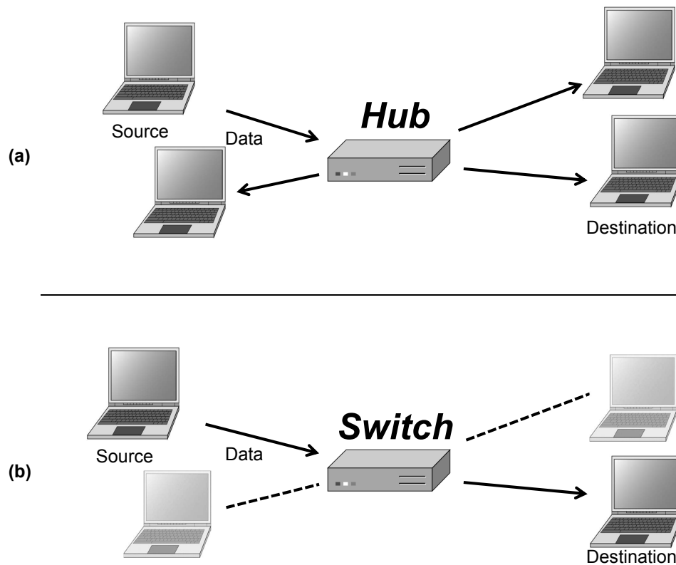
Figure 6: Hub vs. switch: (a) A hub copies and transmits traffic to all attached devices. (b) A switch only transmits frames to the appropriate destination device.
