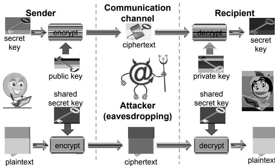
Figure 12: Use of a public-key cryptosystem to exchange a shared secret key, which is subsequently employed for communicating with a symmetric encryption scheme. The secret key is the “plaintext” message sent from the sender to the recipient. © Igor Nazarenko/Shutterstock
