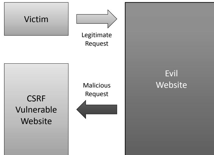
Figure 17: In a CSRF attack, a malicious web site executes a request to a vulnerable site on behalf of a trusted user of that site.
