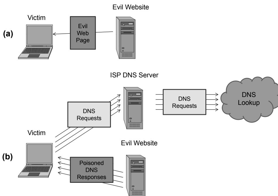
Figure 8: A DNS cache poisoning attack against a client: (a) On visiting a malicious web site, the victim views a page containing many images, each causing a separate DNS request to be made to a nonexistent subdomain of the domain that is to be poisoned. (b) The malicious web server sends guessed responses to each of these requests. On a successful guess, the client's DNS cache will be poisoned.
