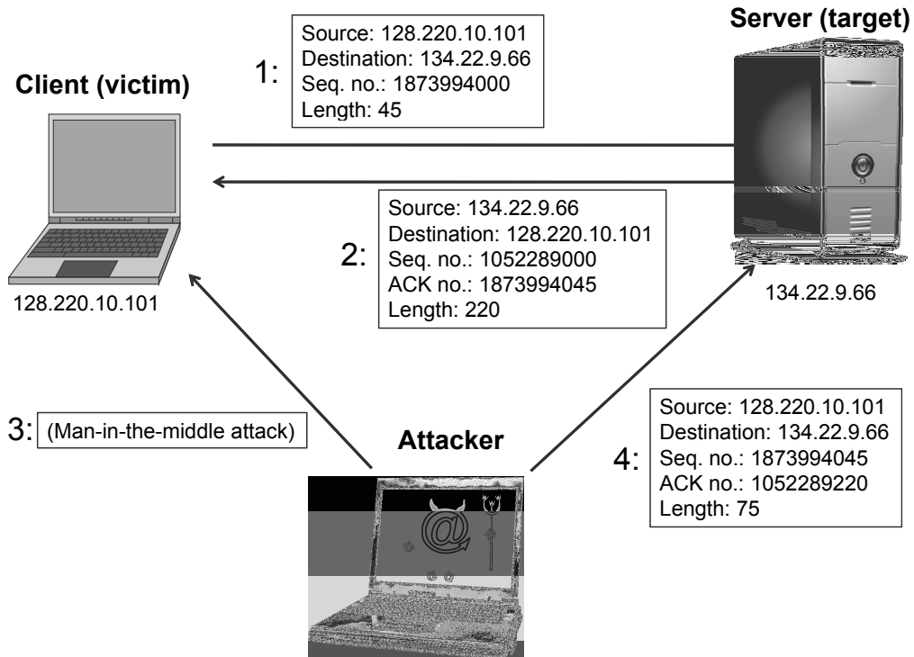
Figure 18: A TCP session hijacking attack. (server) © tatniz/Shutterstock; (laptop computer) © PhotoStocker/Shutterstock
