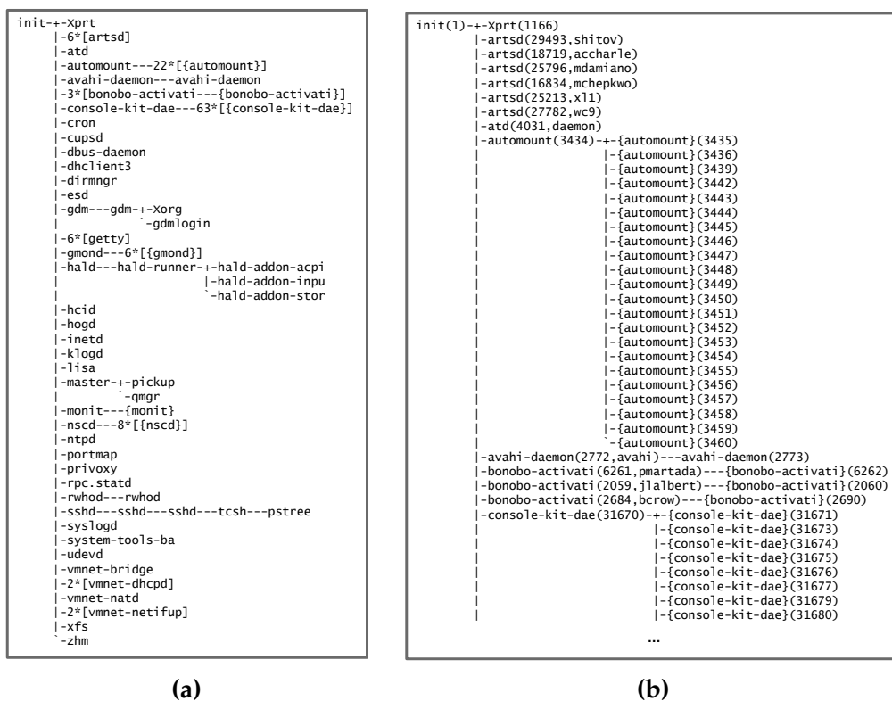
Figure 2: The tree of processes in a Linux system produced by the ps command. The process tree is visualized by showing the root on the upper left-hand corner, with children and their descendants to the right of it. (a) Compact visualization where children associated with the same command are merged into one node. For example, 6*[artsd] indicates that there are six children process associated with artsd , a service that manages access to audio devices. (b) Fragment of the full visualization, which also includes process PIDs and users.
