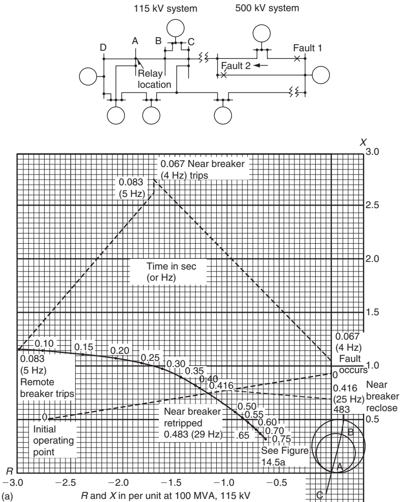
FIGURE 14.5 (a) A 500 kV fault for which the 115 kV system was able to maintain stability. (Continued on next page.)
