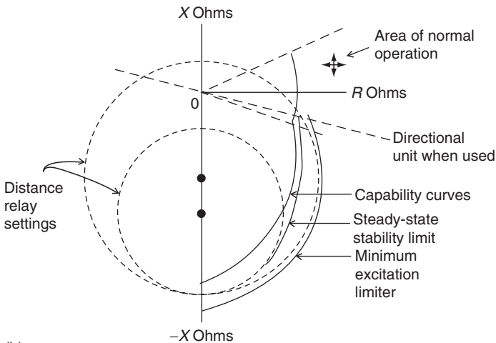
FIGURE 8.17 Typical power capability and stability curves for a generator and their conversion to an R - X diagram for (40) relay protection application; (a) capability and stability curves on power axes; (b) power curves transferred to R - X axes with distance-type relay protection.
