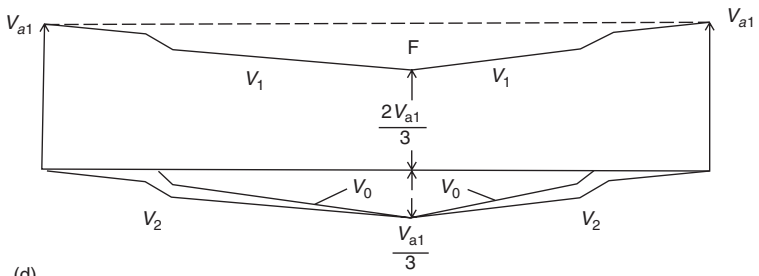
FIGURE 4.31 System sequence voltage profiles during shunt faults: (a) three-phase faults; (b) phase-to-phase faults; (c) two-phase-to-ground faults; (d) phase-to-ground faults.
