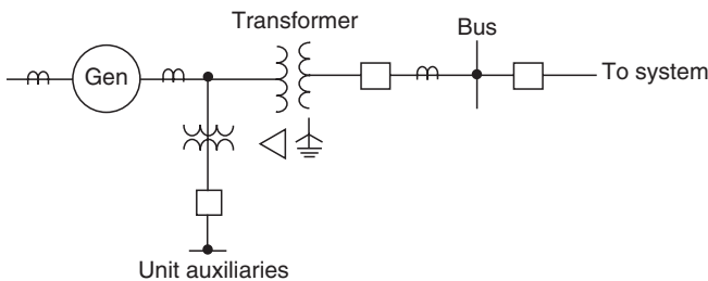
FIGURE 8.4 Unit-connected generator.
