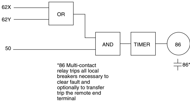
FIGURE 12.28 Typical breaker failure–local backup DC (schematic): (a) typical circuit breaker trip systems and auxiliaries for breaker failure–local backup (where breakers have double trip coils, 94 relay coil, and contact is omitted and the second trip coil 52 TC 2 connected in place of the 94 relay coil); (b) typical contact logic for breaker failure–local backup; (c) typical solid-state logic for breaker failure–local backup.
