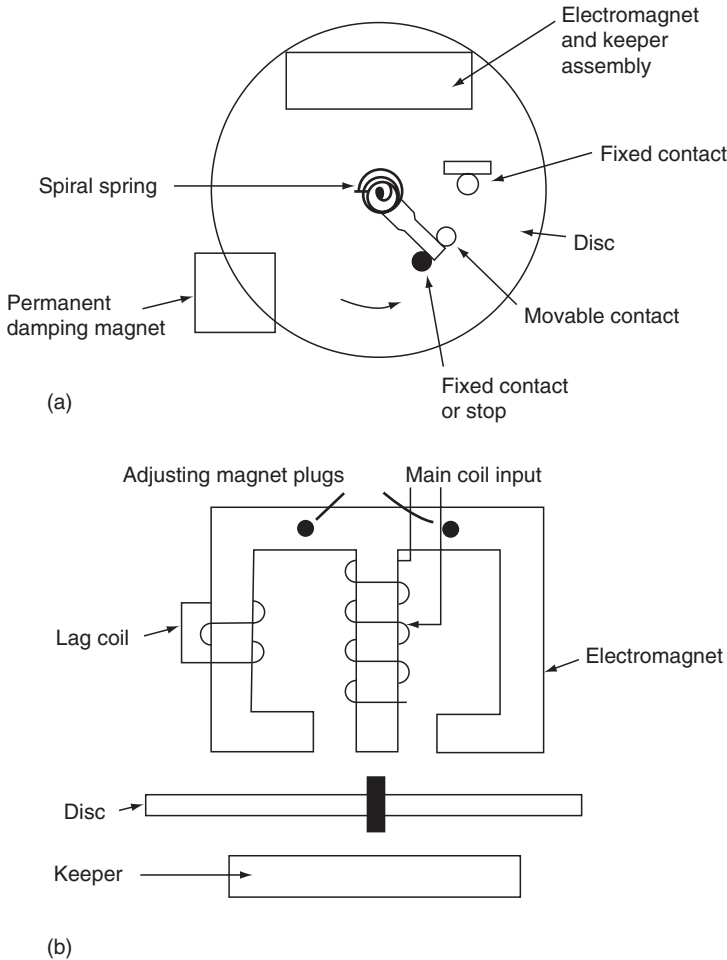
FIGURE 6.6 Typical induction disk inverse-type-overcurrent or voltage relay: (a) top view; (b) side view.
